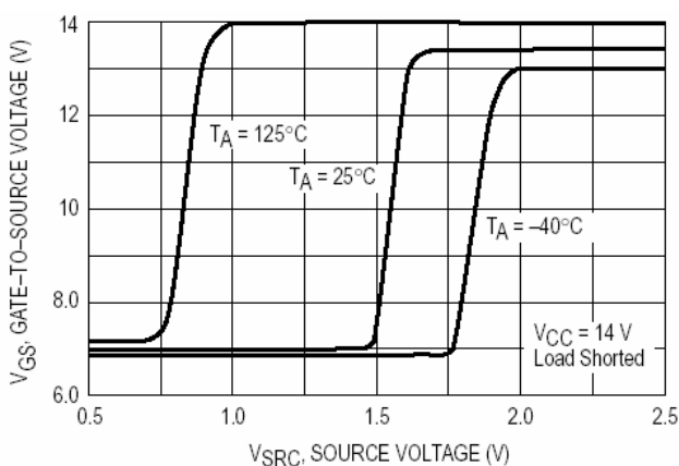
Figure 18. Gate-to-Source Voltage versus Source Voltage
