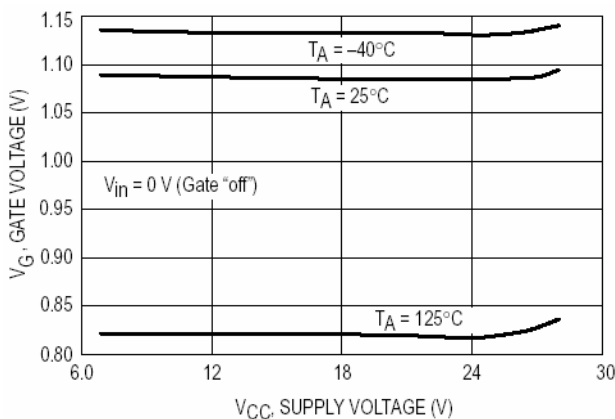
Figure 16. Gate Voltage versus Supply Voltage
