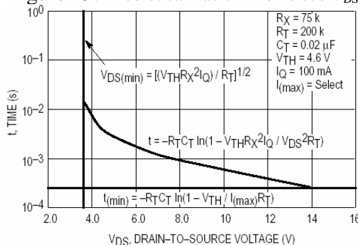
Figure 29. Theoretical Fault Time versus V_{DS} (7)
