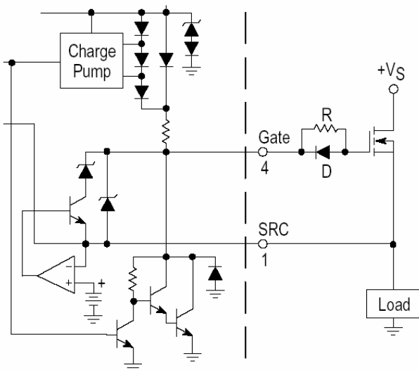
Figure 31. Slow Down FET Turn-On
