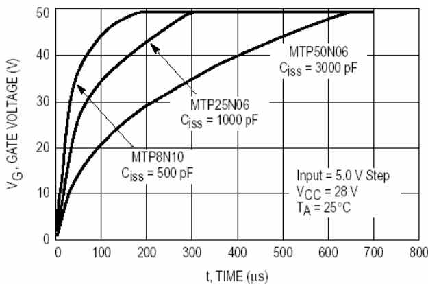
Figure 26. FET Comparison Gate Response
