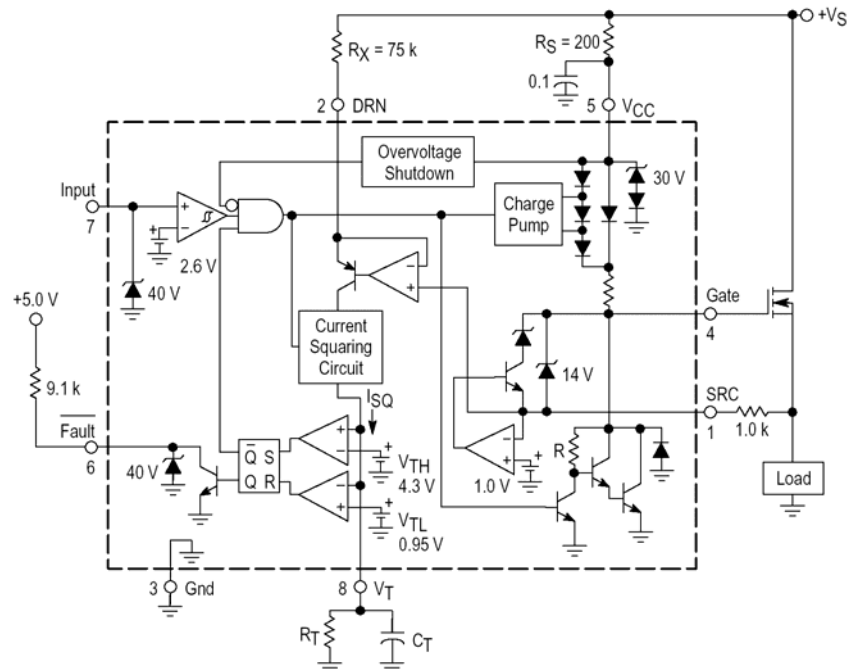
Figure 1. Typical Application
