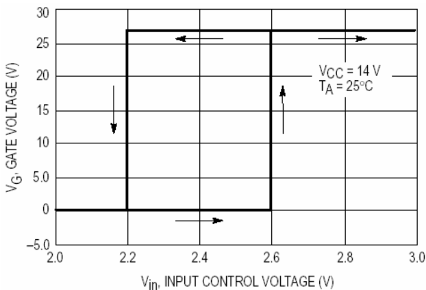
Figure 14. Gate Voltage versus Input Control Voltage
