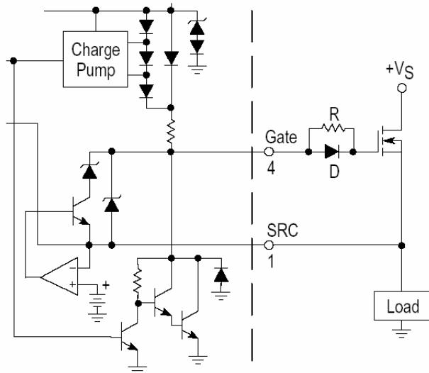
Figure 32. Slow Down FET Turn-Off
