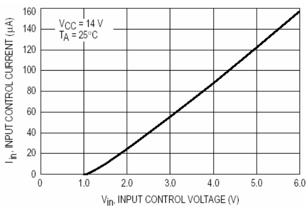
Figure 4. Input Control Current versus Input Control Voltage
