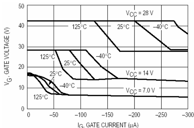
Figure 17. Gate Voltage versus Gate Current
