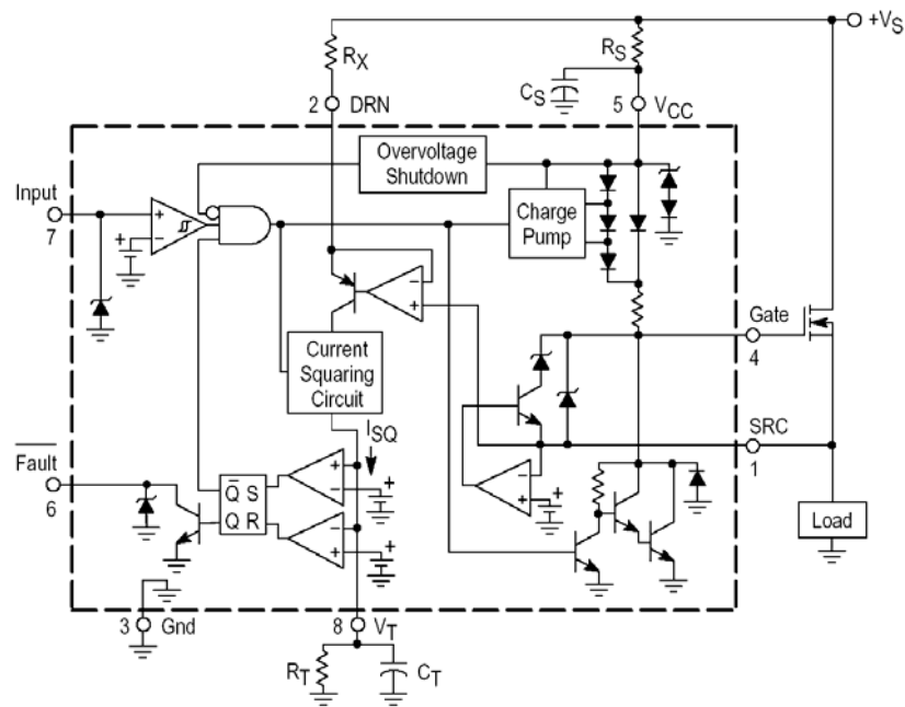
Figure 1. Typical Application
