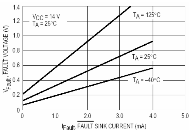
Figure 6. Fault Voltage versus Fault Sink Current
