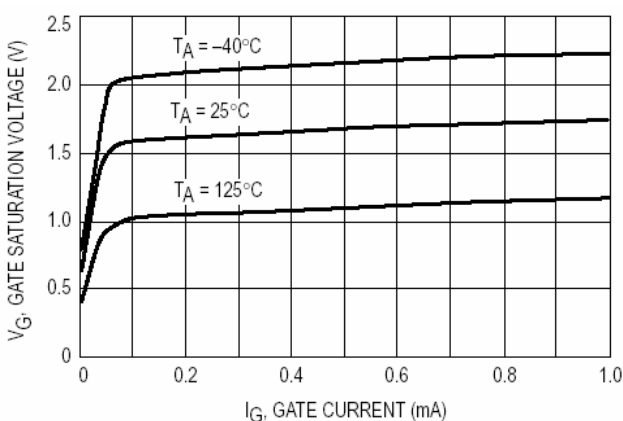
Figure 20. Gate Saturation Voltage versus Gate Current
