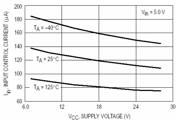
Figure 5. Input Control Current versus Supply Voltage
