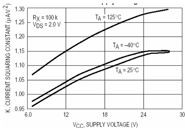
Figure 7. Squaring Constant “K” versus Supply Voltage
