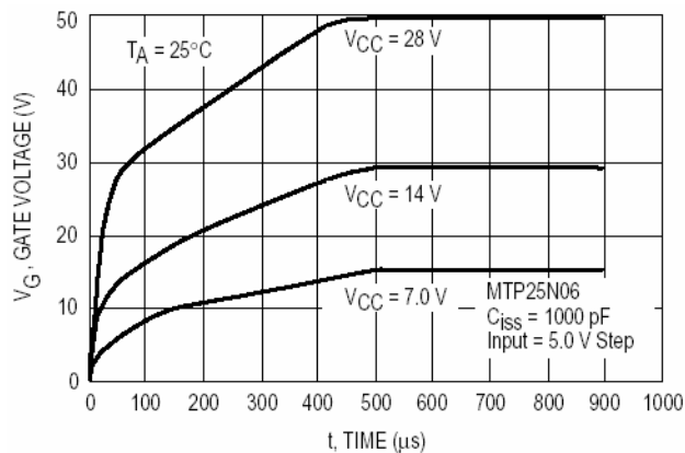
Figure 27. MTP25N06 Gate Response
