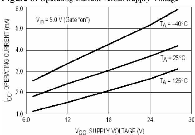
Figure 3. Operating Current versus Supply Voltage
