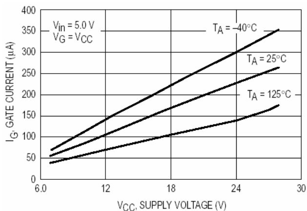
Figure 19. Gate Current versus Supply Voltage
