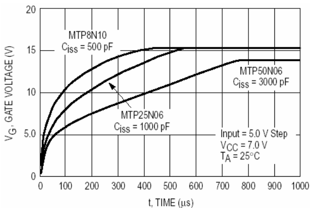
Figure 24. FET Comparison Gate Response
