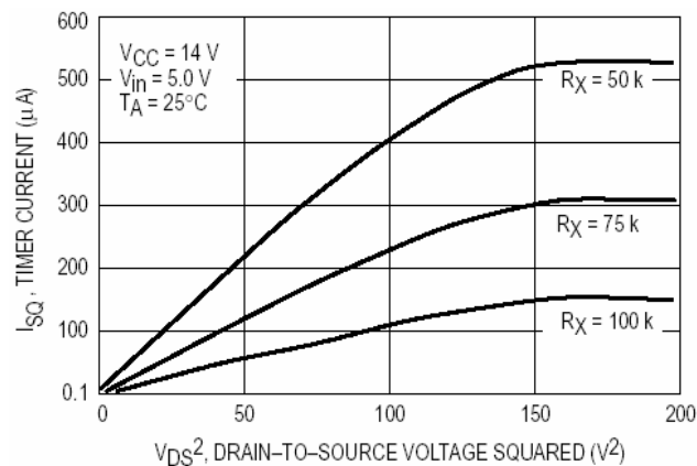
Figure 9. Timer Current versus Drain-to-Source Voltage Squared
