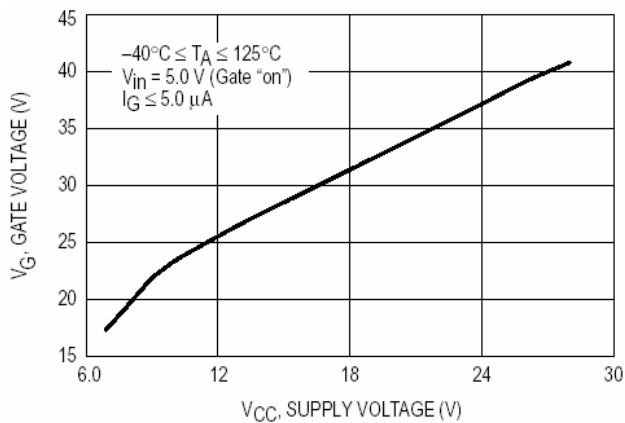
Figure 15. Gate Voltage versus Supply Voltage
