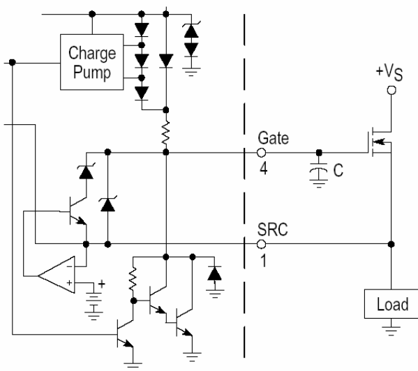
Figure 33. Slow Down Turn-On and Turn-Off of FET
