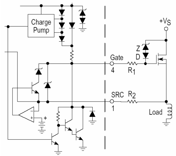
Figure 36. Overvoltage Protection of FET
