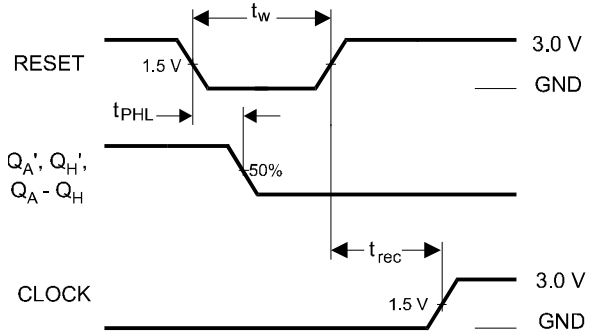
Figure 2. Switching Waveform
