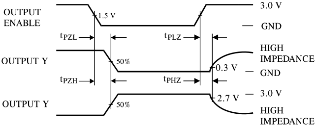
Figure 3. Switching Waveforms
