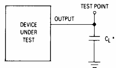
Figure 2. Test Circuit
